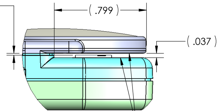
DETAIL A SCALE 2 : 1 No Draft
